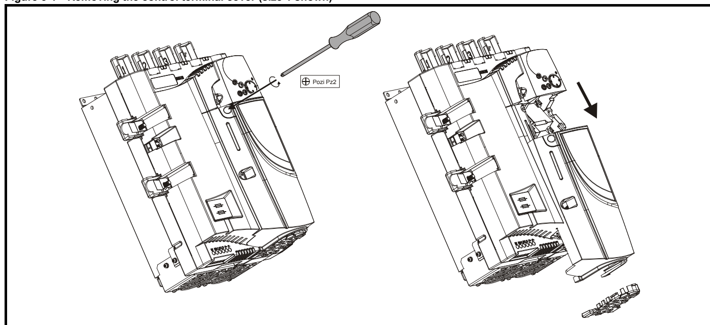
Figure 3-1 Removing the control terminal cover (size 1 shown)
